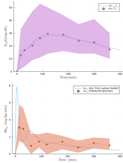
(b) Results of the model fitting the oral bolus after intestinal resection dataset.
