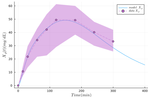
(a) Results of the model fitting the oral bolus dataset
